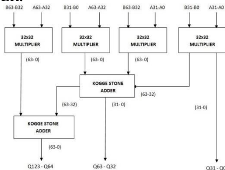
Fig 1.11 :64-bit Vedic multiplier using Kogge Stone Adder
