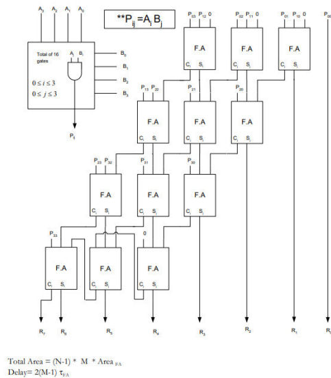
Fig 1.1: array multiplier
