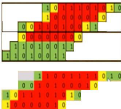
Fig 1.6 :partial products addition,step2
