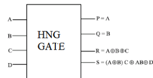
Fig 4.6: HNG Gate
