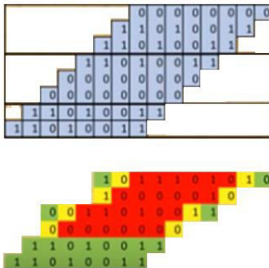
Fig 1.5: partial product addition ,step1
