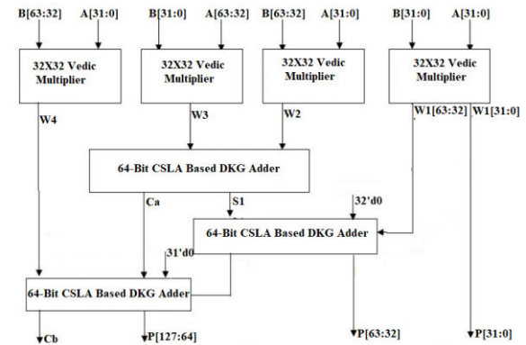
Fig 4.15 : proposed Vedic Multiplier
