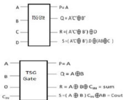
Fig 4.5 shows a 4*4 TSG gate.
