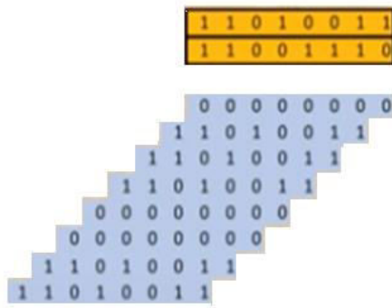
Fig 1.4: Stage1 partial products
