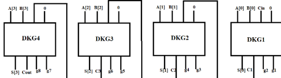
Fig 4.8: bit RCA based DKG adder
