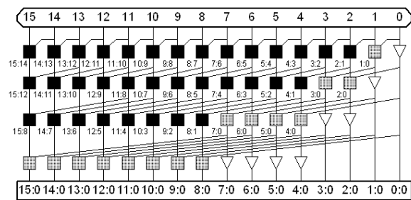
Fig 1.12 -16 bit Kogge Stone Adder
