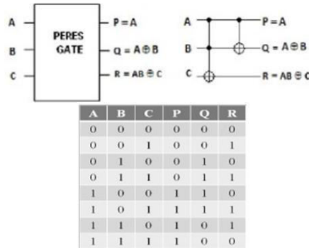
Fig 4.4: shows a 3*3 Peres gate.
