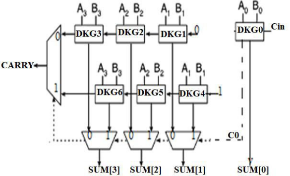
Fig 4.14 :4-BIT DKG ADDER
